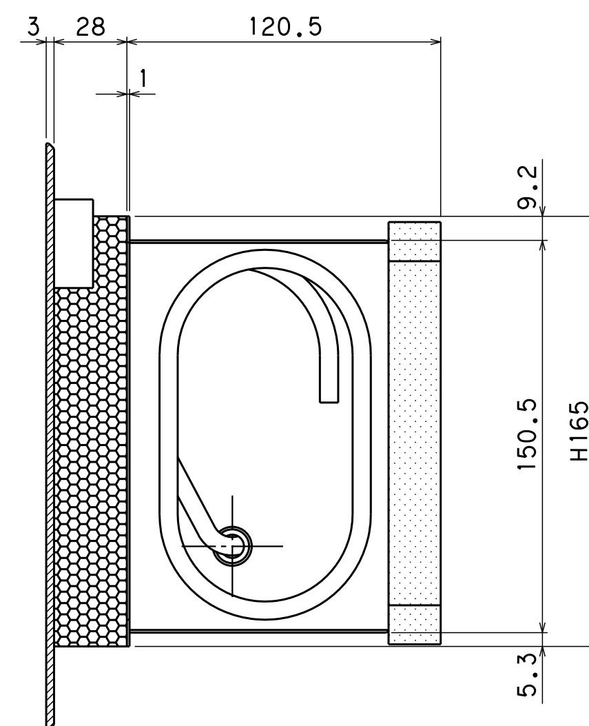
ZAA187-BA01 FLATFAN 商品図(柱105)
