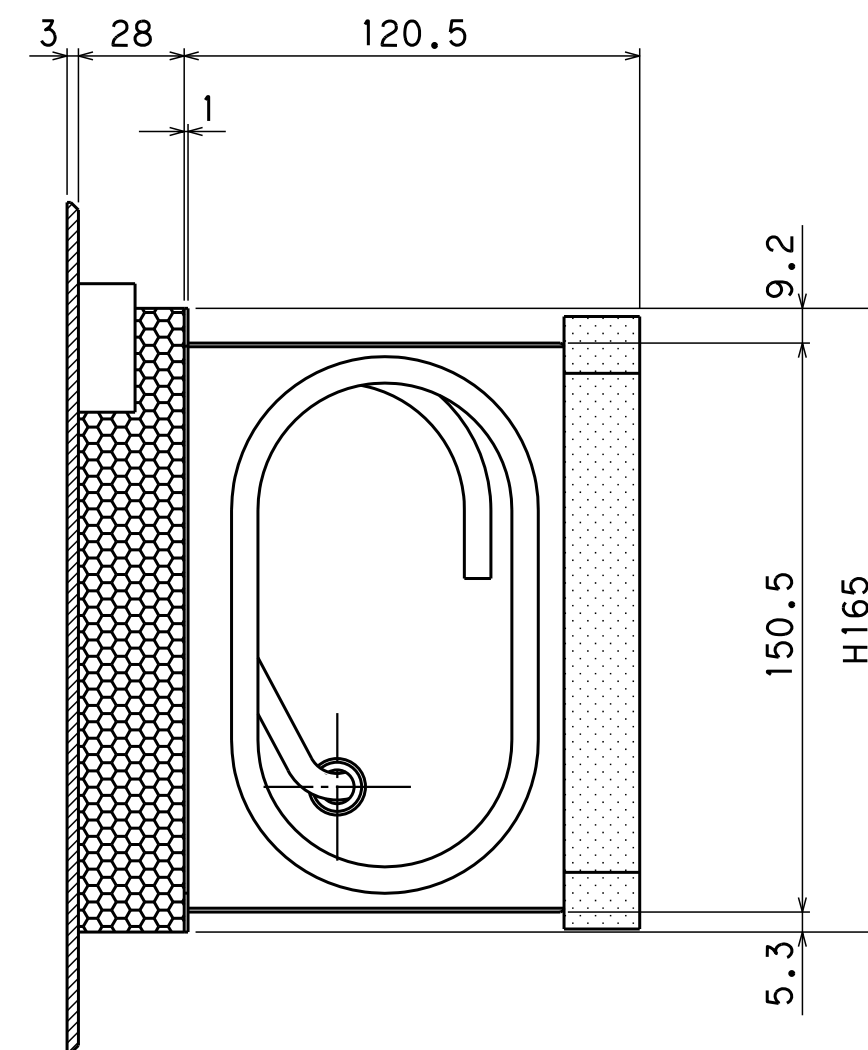
ZAA187-BB01 FLATFAN 商品図(柱120)
